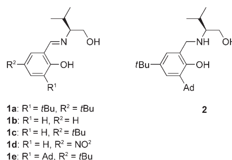
Scheme 1. Chiral ligands used in the study. Ad = adamantyl.
